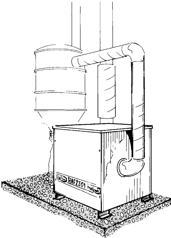
Installation Example: RAF 2501 and S 34000
