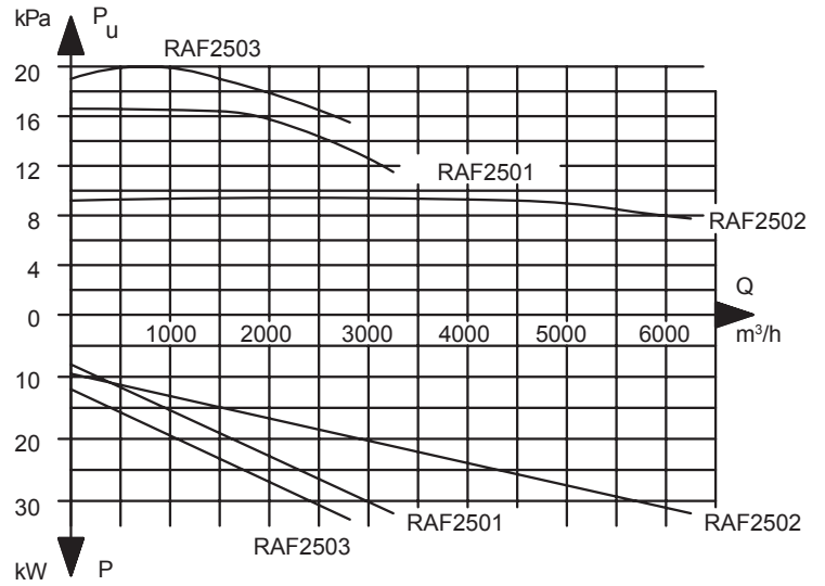
Figure shows available capacity in an extraction system, see explanation on page 7
